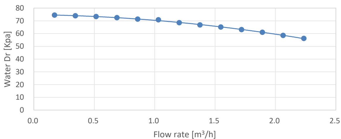
AW102MUGHA/AW10NMUGHA Water Pressure External Residual Pressure
