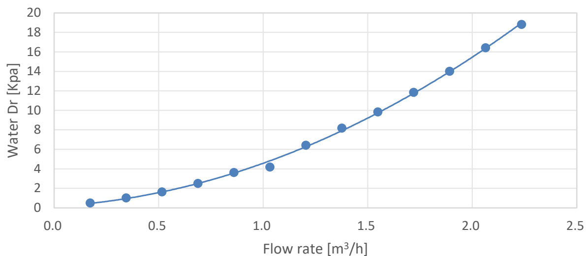
AW102MUGHA/AW10NMUGHA Water Pressure Drop
