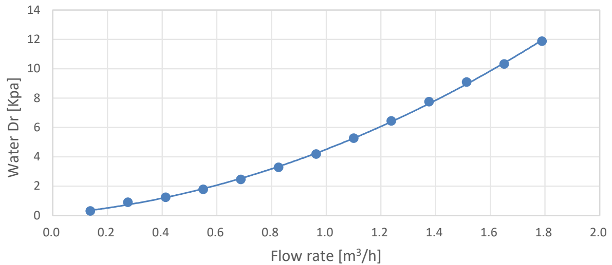
AW082MUGHA Water Pressure Drop
