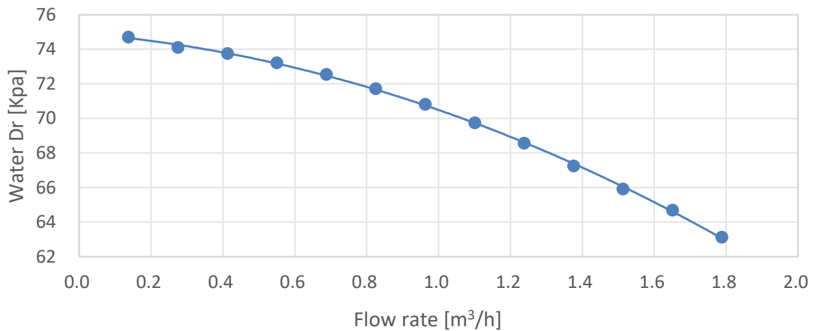
AW082MUGHA Water Pressure External Residual Pressure
