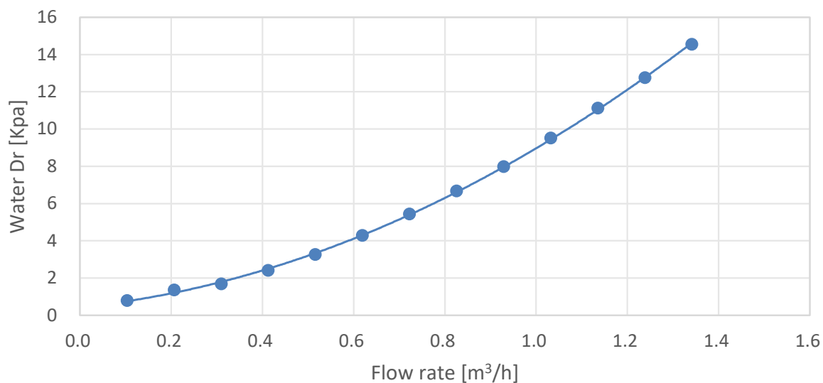
AW062MUGHA Water Pressure Drop
