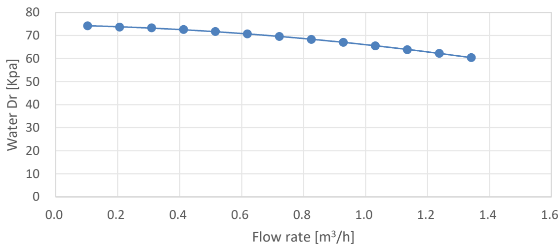
AW062MUGHA Water Pressure External Residual Pressure
